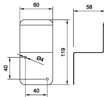
Mount bracket, 1.2mm stainless steel
