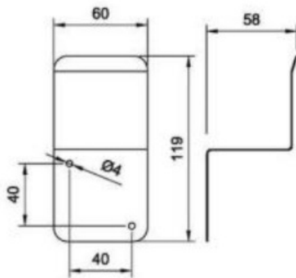
Mount bracket, 1.2mm stainless steel
