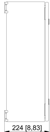
LEFT VIEW
