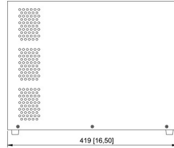
BATTERY SIDE VIEW
