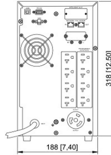
BATTERY REAR VIEW
