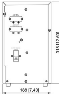
BATTERY REAR VIEW
