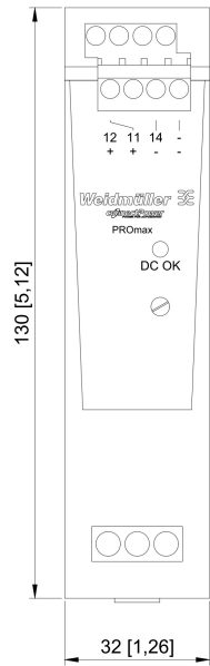
FRONT VIEW
