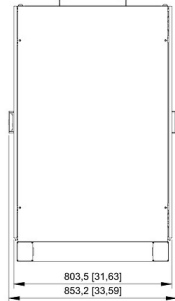
RIGHT VIEW
