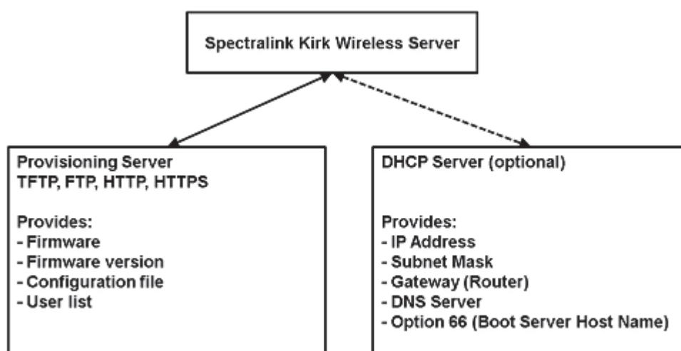
Figure 1 Provisioning Architecture
